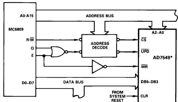
Figure 8. AD7549-MC6809 Interface
